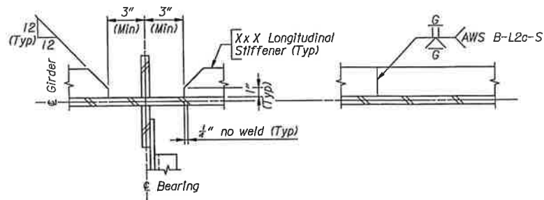
SECTION THRU BEARING STIFFENERS AT EXTERIOR GIRDERS
