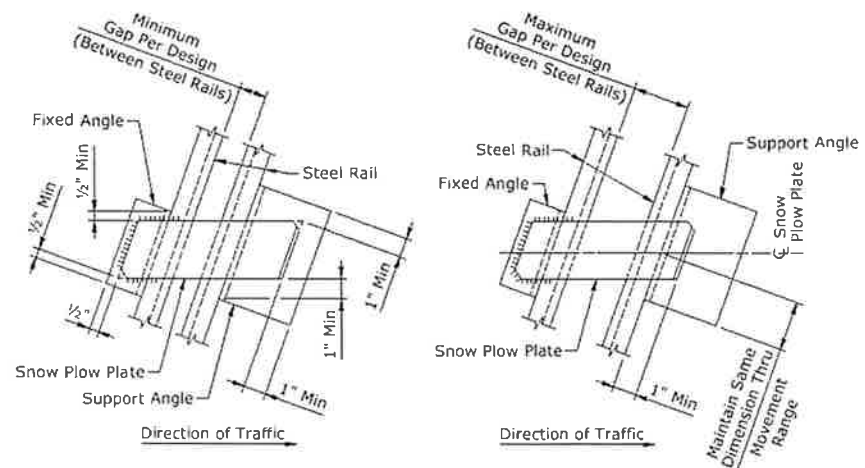
SKETCH FOR SNOW PLOW PLATE ASSEMBLY SIZING
