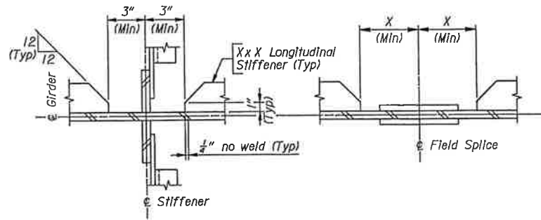
SECTION THRU INTERMEDIATE OR BEARING STIFFENERS
