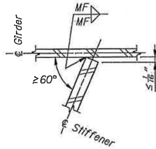
CASE I (Stiffener not beveled)
