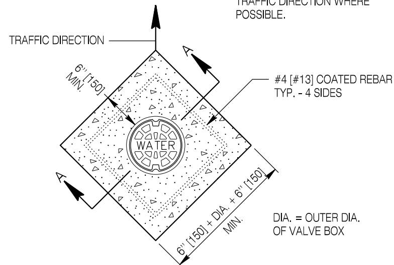
VALVE BOX COLLAR
