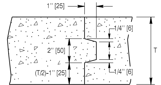
TYPICAL KEYWAY DETAIL
