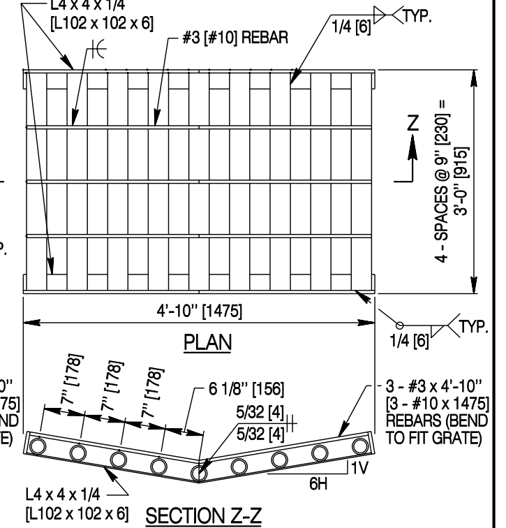
TYPE 3 GRATE
