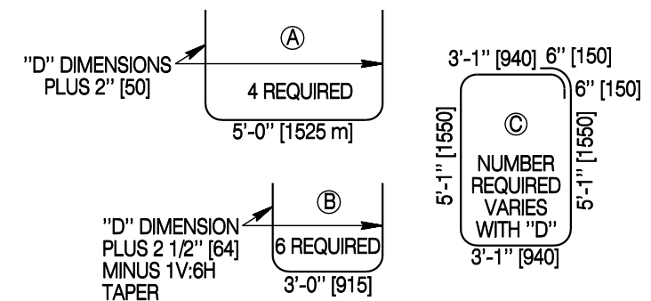
TYPE 2 GRATE
