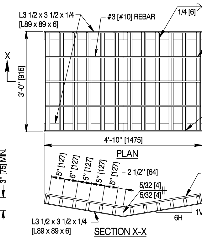
TYPE 1 GRATE
