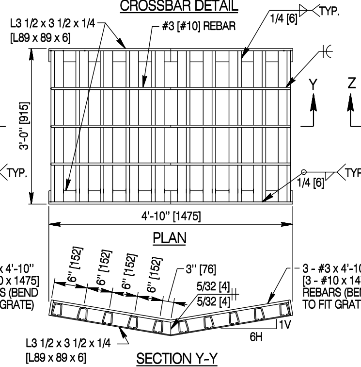
TYPE 2 GRATE
