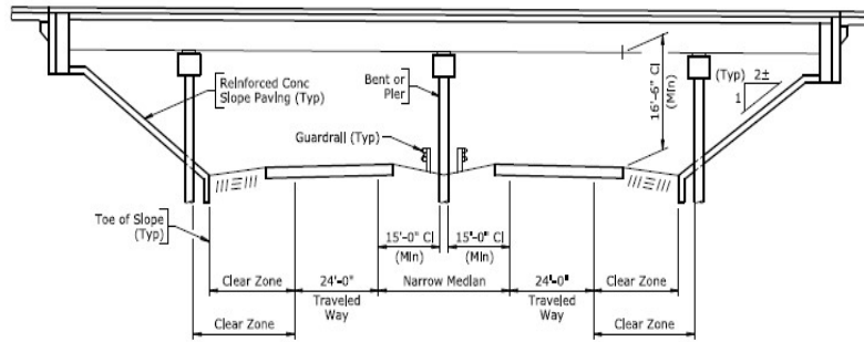
INTERSTATE HIGHWAY UNDERPASS Narrow Median - 60'-0" or less
