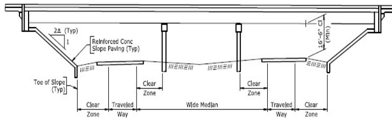
INTERSTATE HIGHWAY UNDERPASS Wide Median - Over 60'-0"
